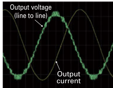
Current and Voltage Output Waveforms for 3.3 kV Drive
