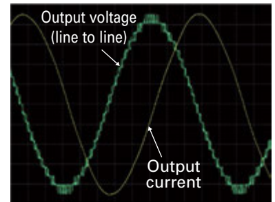
Current and Voltage Output Waveforms for 6.6 kV Drive
